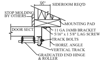
WOOD JAMB DETAIL (TYPICAL) SECTION 'B-B'
