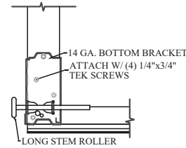
BOTTOM BRACKET DETAIL DETAIL 2/SI.1
