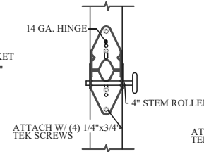
END HINGE DETAIL DETAIL 3/SI.1
