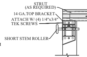
TOP BRACKET DETAIL DETAIL 1/SI.1
