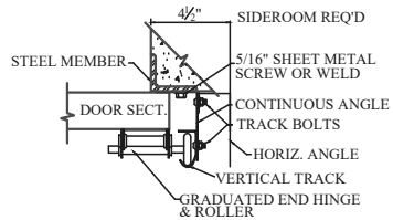
STEEL JAMB DETAIL (TYPICAL) SECTION 'B-B'
